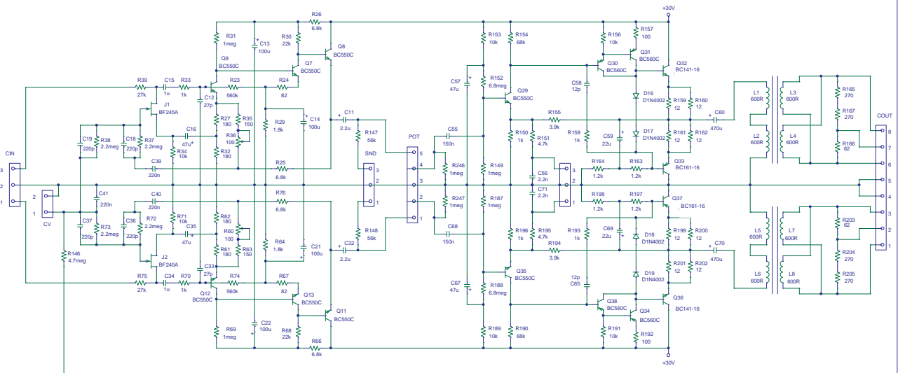
JH. FC2 Stereo Compressor Based on Urei 1176 (c) J. Haible 2001 Part 1
