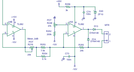
JH. FC2 Stereo Compressor Based on Urei 1176 (c) J. Haible 2001 Part 1
